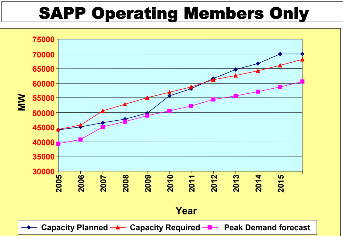
Graph 2: SAPP Demand Supply Situation (Operating SAPP Members Only).
